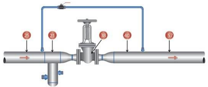
Figure 4: Downstream Ultrasound
