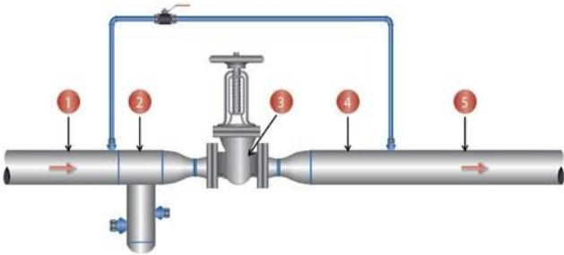
Figure 2: Main Valve Test with Equal Readings
