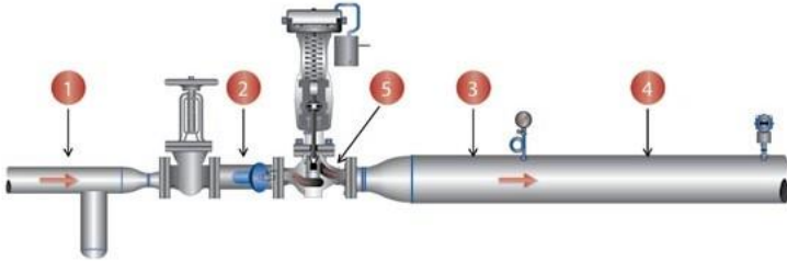
Figure 6: Control Valve Testing
