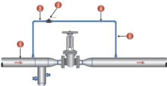
Figure 3: Main Valve Leaking
